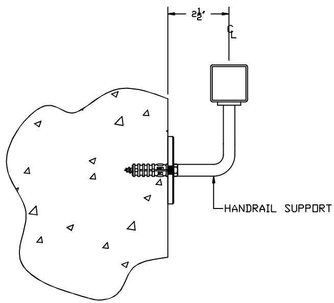
STANDARD WALL BRACKET
